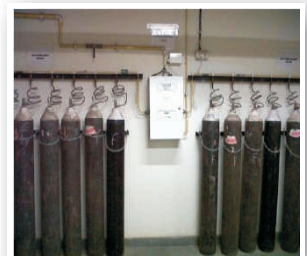
5+5 Manifold
